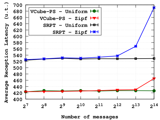
Fig. 7. Average reception latency with 256 nodes and 128 topics.
