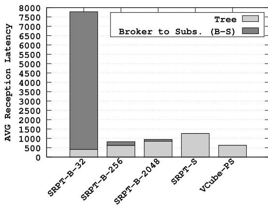
Fig. 9. Average reception latency for different approaches and 4096 nodes.
