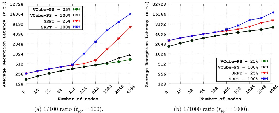
Fig. 5. Reception latency with 25% and 100% of publishers (log scale).
