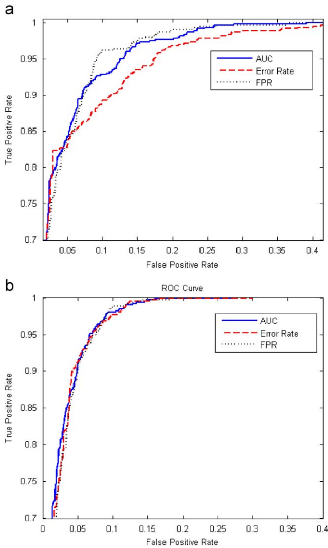
Fig. 10. Comparison among the three objective functions considered in this work. (a) Sk = 5 and (b) Sk = 15 . The validation set II was considered here.
