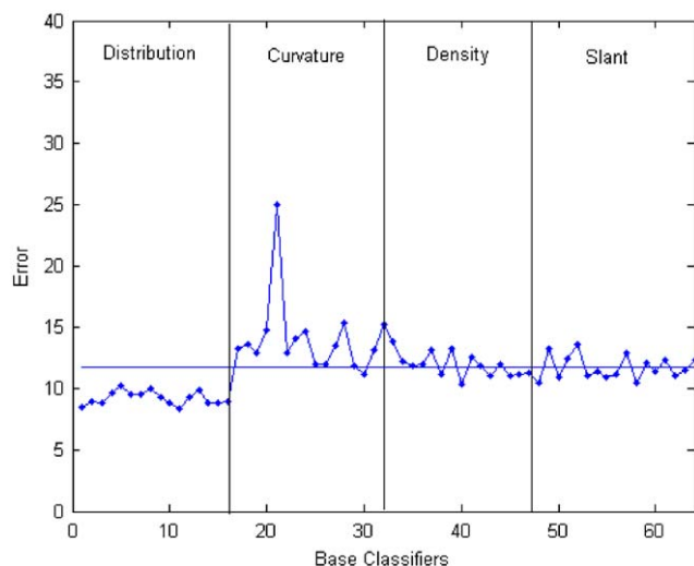
Fig. 9. Performance of the base classifiers.
