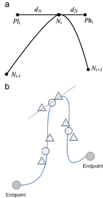
Fig. 8. (a) Example of the features extracted from a segment and (b) example of the points detected in a real segment extracted from the signature of the Fig. 7b
