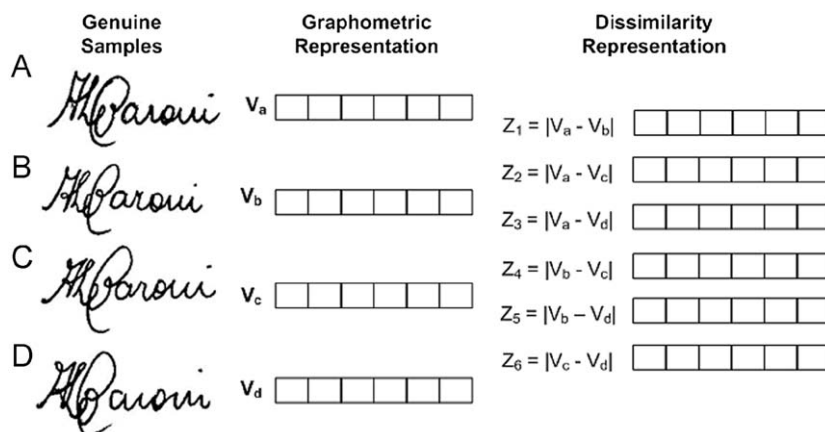
Fig. 3. Dissimilarities among genuine samples of the same writer to generate the positive samples. From four genuine samples, six dissimilarity vectors are created.
