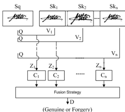
Fig. 2. Architecture of the global approach.
