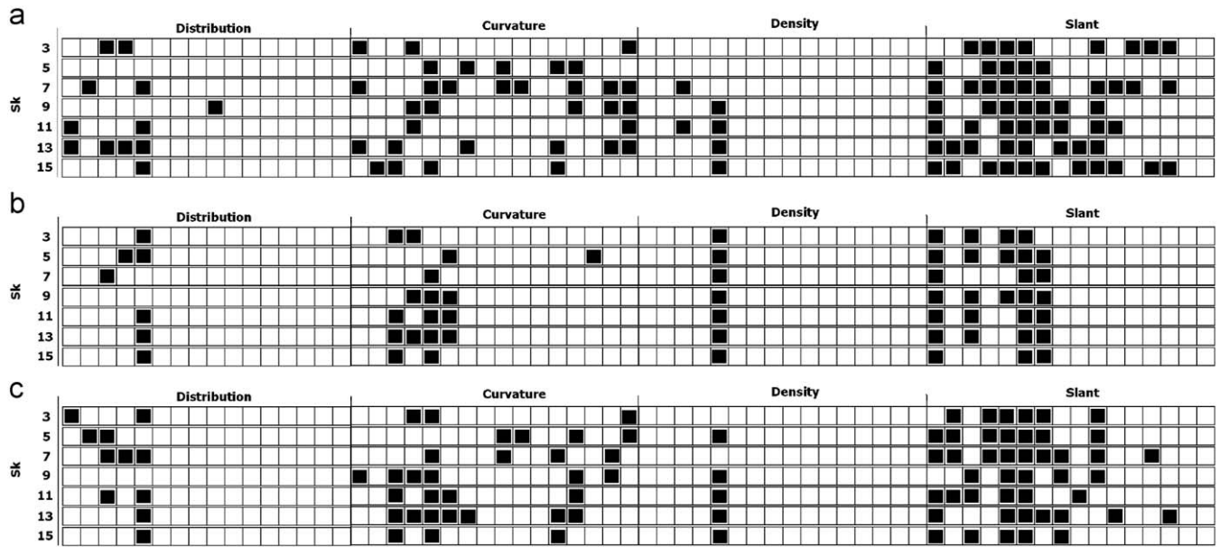
Fig. 12. Classifiers selected during the search using validation set I and fitness: (a) overall error, (b) AUC, and (c) FPR fixed at 10%.
