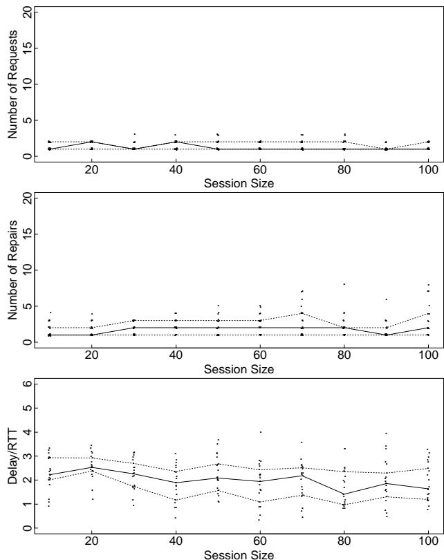
Figure 10: Adaptive algorithm on round 40, for a bounded-degree tree of 1000 nodes with degree 4 and a randomly picked congested link.
