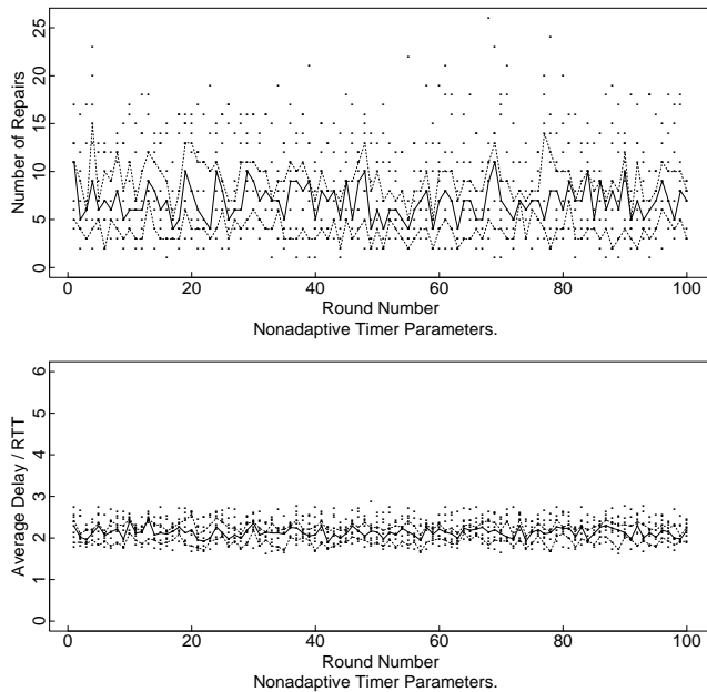
Figure 8: The non-adaptive algorithm.
