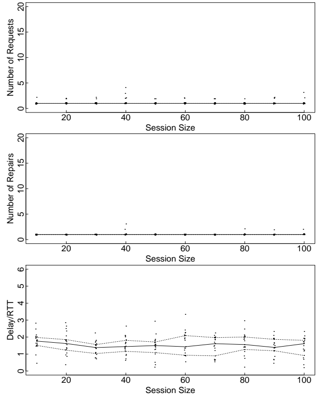
Figure 3: Random trees with a random congested link, where all nodes are members of the multicast session.
