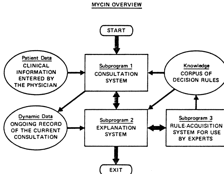
FIG. 1. Diagram demonstrating the flow of control and the flow of information within the MYCIN System. The three subprogram components are enclosed in boxes. Control passes from one subprogram to another as shown by the heavy arrows. Light arrows indicate program access to information used by the system. The program's knowledge base is contained in the corpus of rules shown on the right. Each rule is of the form:
