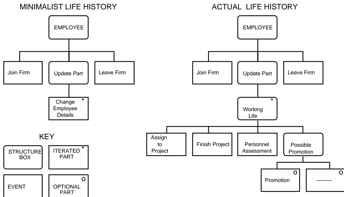
Figure 4.2: Minimalist & More Complex Entity Life Histories
