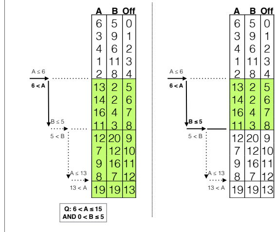
Fig. 2: A search with predicates 6 < A \leq 15 AND 0 < B \leq 5 in the Adaptive KD-Tree.
