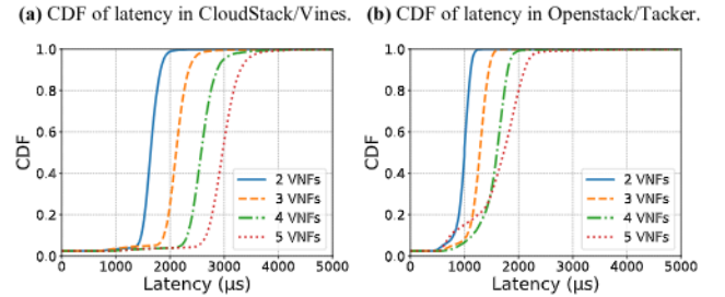
Figure 11. CDF of the latency of the SFCs.
