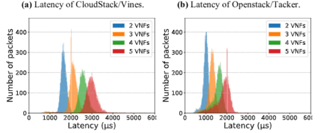
Figure 10. SFC latency distribution in microseconds.
