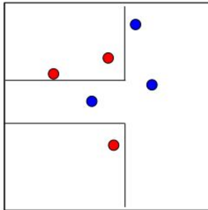
Combined classifier
